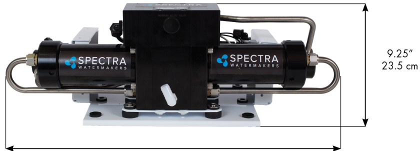
High Pressure Clark Pump and Membrane Depth 12" / 30.5 cm
