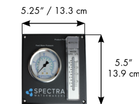
Remote Monitoring Panel Depth 1.63" / 4.1 cm
